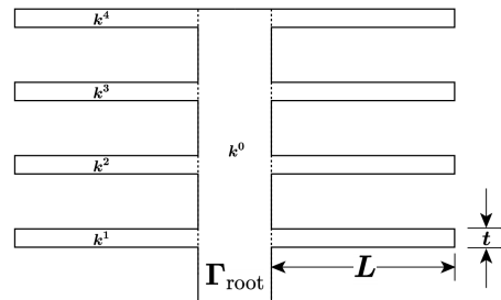
FIG. 1. Thermal fin geometry.
