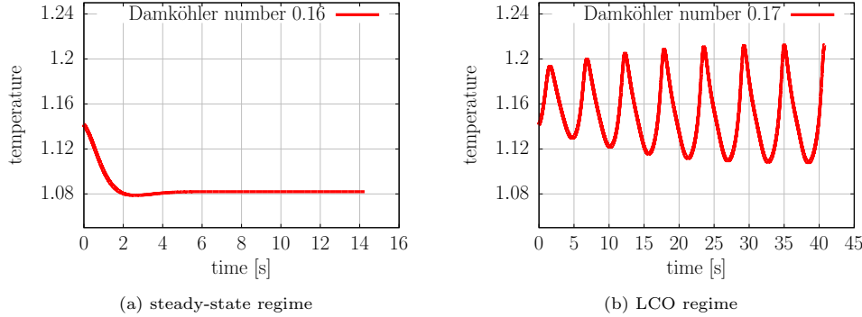
FIGURE 8. Tubular reactor: If the input z < z^* is below the critical parameter z^* \in \mathcal{D} , the temperature and the concentration of the tubular reactor converge to a steady state as shown in (a) for the temperature at 1 \in \Omega . If z > z^* , the tubular reactor enters an LCO as plotted in (b).
