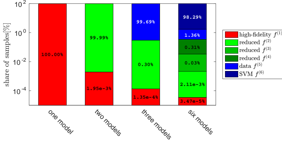
FIGURE 6. Plate model : The plot reports how Algorithm 2 distributes the total number of samples across the high-fidelity, the reduced, the data-fit, and the SVM models for the MFMC estimator with two, three, and six models. Note the logarithmic scale on the y-axis.
