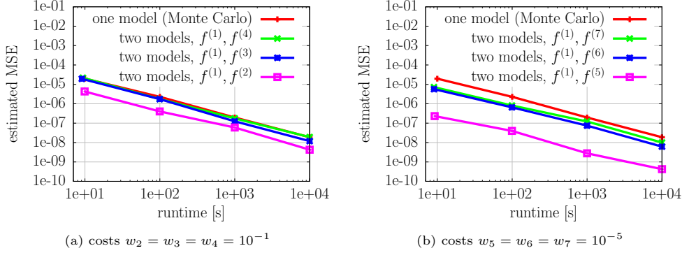
FIGURE 11. Short column: The plots in (a) and (b) show that even surrogate models with low correlation coefficients can lead to runtime speedups if the costs are low.
