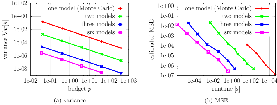
FIGURE 5. Plate model: The plot in (a) shows the variance of the MFMC estimator with two (high-fidelity f^{(1)} , reduced f^{(2)} ), three (high-fidelity f^{(1)} , reduced f^{(2)} , data-fit f^{(5)} ), and all six models f^{(1)}, \dots, f^{(6)} (high-fidelity f^{(1)} , reduced f^{(2)} , f^{(3)} , f^{(4)} , data-fit f^{(5)} , and SVM f^{(6)} ). Compared to the Monte Carlo method with the high-fidelity model only, a variance reduction of about four orders of magnitude is achieved. This is similar to the speedup obtained with the MFMC estimator shown in (b).
