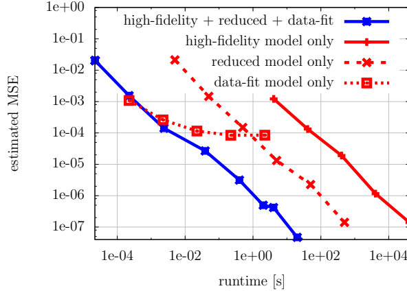
FIGURE 4. Plate model: The MFMC estimator combines the high-fidelity model f^{(1)} , the reduced model f^{(2)} , and the data-fit model f^{(5)} to estimate the expectation of the deflection of the damaged plate. The runtime to derive an MFMC estimate is four orders of magnitude lower than the runtime to obtain the Monte Carlo estimate of comparable accuracy that uses the high-fidelity only. Furthermore, the runtime of the MFMC estimator is two orders of magnitude lower than using the Monte Carlo method with the reduced model f^{(2)} .
