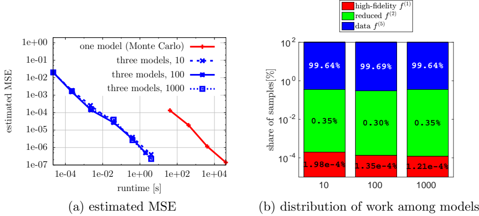
FIGURE 7. Plate model: We use the sample variances and sample correlation coefficients to determine the number of model evaluations m and the coefficients \alpha . The plot in (a) compares the estimated MSE of our MFMC estimators (with models f^{(1)} , f^{(2)} , f^{(5)} ) obtained from the sample variances and sample correlation coefficients from 10, 100, 1000 samples, respectively, see Table 2. The plot indicates that small perturbations in the sample correlation coefficients have a small effect on the MSE of the MFMC estimators. The plot in (b) confirms that small perturbations in the sample estimates lead to small changes in the number of model evaluations.
