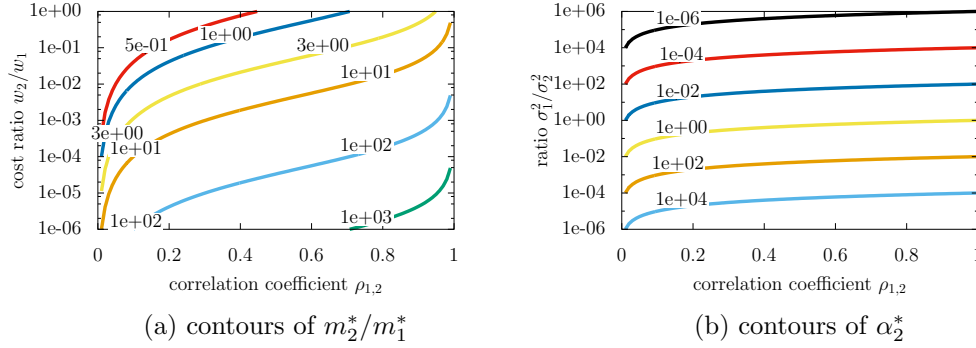
FIGURE 2. The plots show that for an example with two models the number of model evaluations \mathbf{m}^* = [m_1^*, m_2^*]^T and the coefficient \alpha_2^* vary smoothly with respect to the costs w_1, w_2 , the correlation coefficient \rho_{1,2} , and the variances \sigma_1^2, \sigma_2^2 . In particular, small perturbations in the quantities w_1, w_2, \rho_{1,2}, \sigma_1^2, \sigma_2^2 lead to small changes in \mathbf{m}^* and \alpha_2^* .
