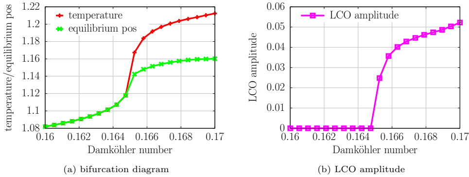
FIGURE 9. Tubular reactor: The bifurcation diagram in (a) visualizes the two regimes of the tubular reactor. The LCO amplitude as shown in (b) is the difference between the temperature and the equilibrium position.
