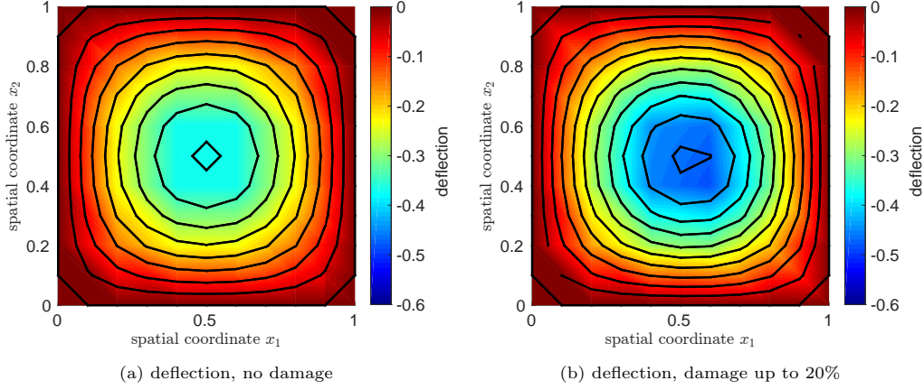
FIGURE 3. Plate problem: A local damage at \mathbf{x}^* = [0.7, 0.4]^T \in \Omega leads to a larger deflection of the plate.
