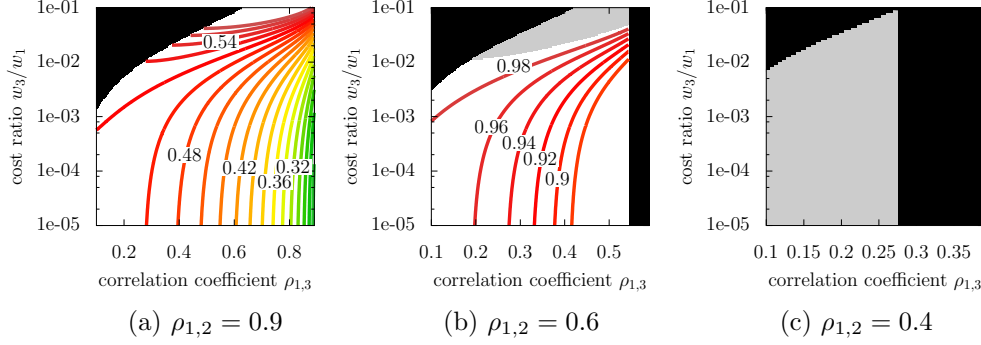
FIGURE 1. The plots show the contours of the variance reduction ratio (3.23) of an MFMC estimator with three models f^{(1)}, f^{(2)}, f^{(3)} . The black region shows where condition (3.12) is violated and the gray region where the MFMC estimator leads to a higher variance than the Monte Carlo estimator. The plots confirm that the variance reduction of the MFMC estimator is determined by the properties of the collective whole of the models, and not by the properties of each model separately.
